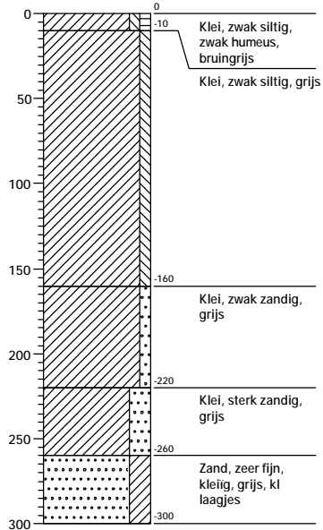
Boring: 16
