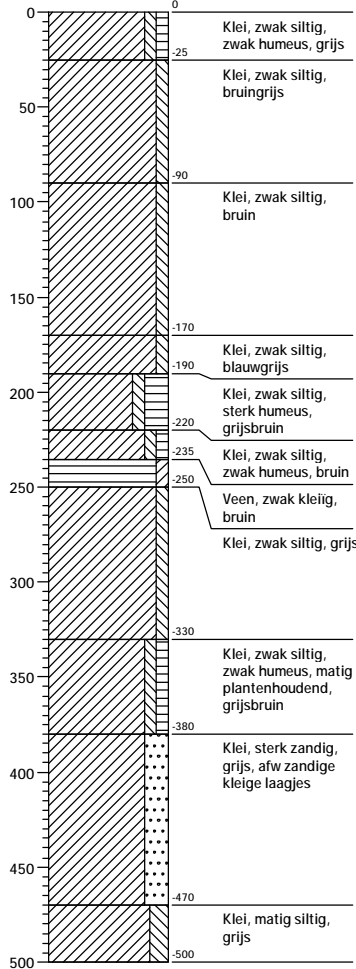
Boring: 01
