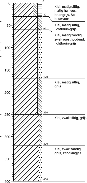
Boring: 25
