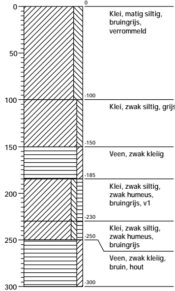
Boring: 21
