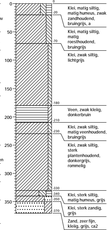
Boring: 39
