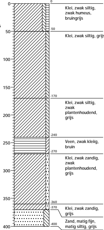
Boring: 03
