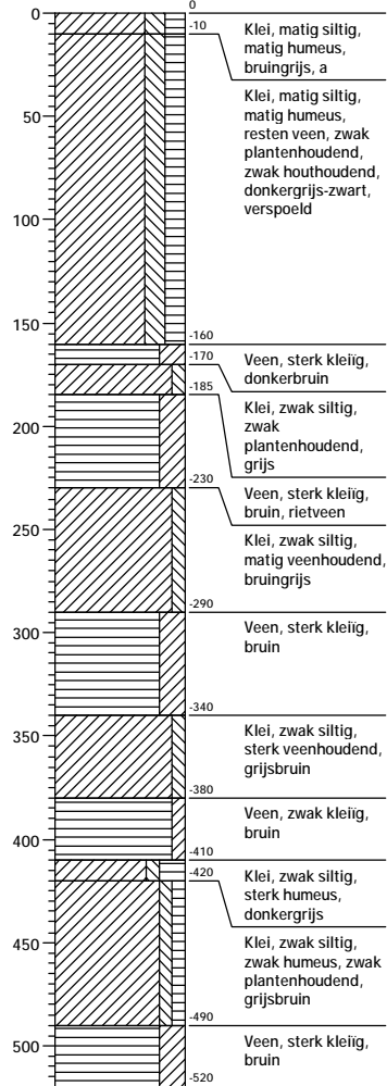
Boring: 36
