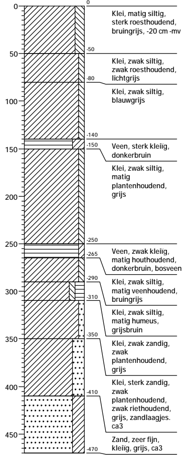
Boring: 38
