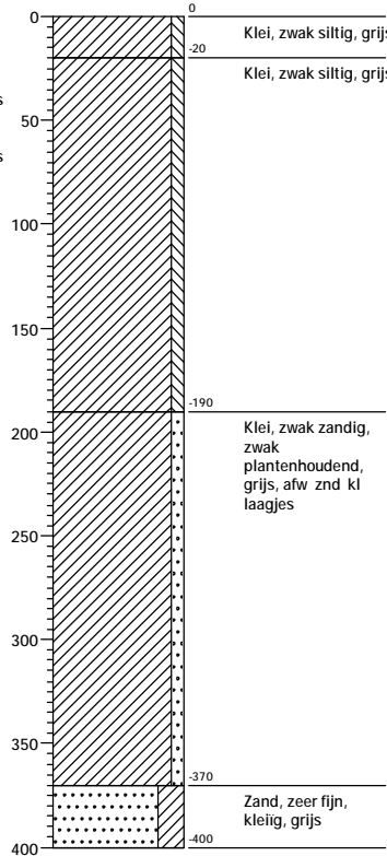
Boring: 18
