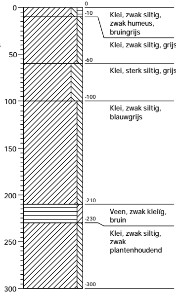
Boring: 17
