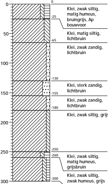
Boring: 22
