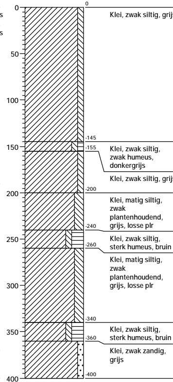
Boring: 19
