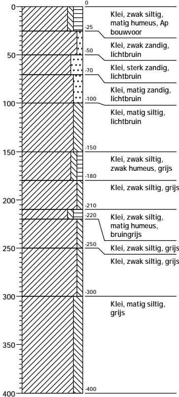
Boring: 23
