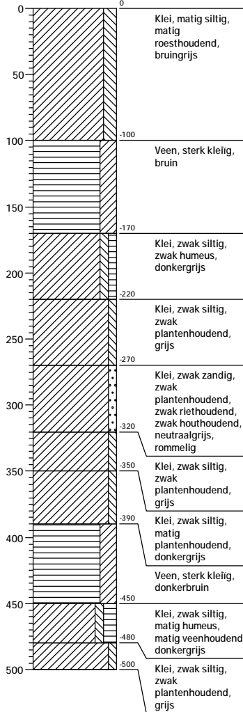
Boring: 37
