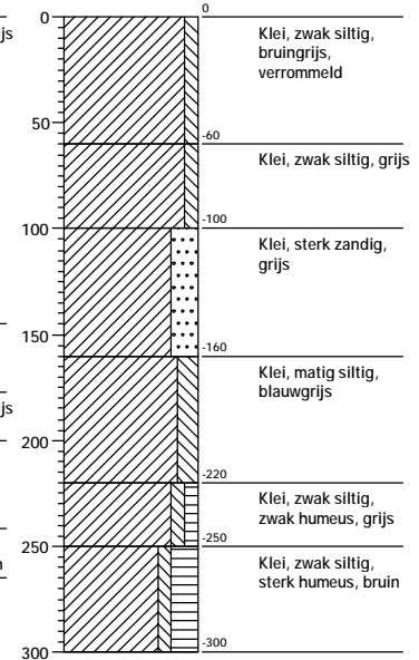
Boring: 20
