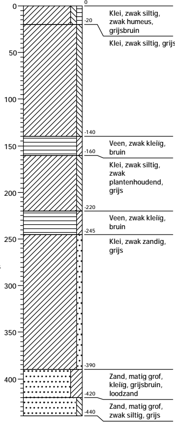
Boring: 02
